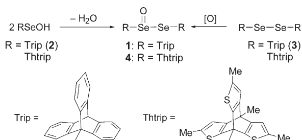
Scheme 1. Formation of selenoseleninates from selenenic acids and diselenides.
